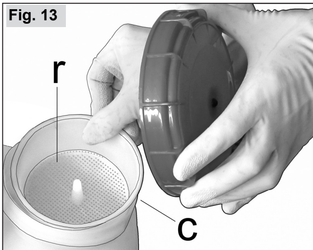
The basket in the filling neck (c) of the liquid tank contains a filter screen (r).
