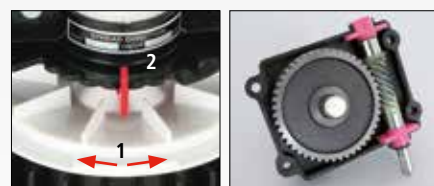
Adjustable throw direction (1), agitator (2) Enclosed worm drive with angular metal gears
