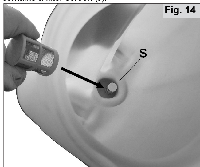
The intake screen (s) is pushed on at the intake hose to the pump of the spraying agent tank.
