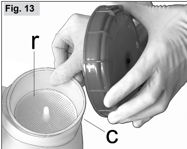
The basket in the filling neck (c) of the liquid tank contains a filter screen (r).
